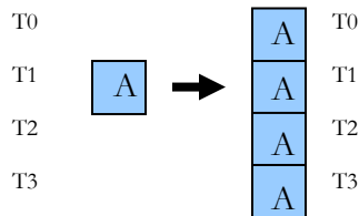
Figure 7.1-1 upc_all_broadcast
