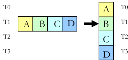
Figure 7.1-2 upc_all_scatter
